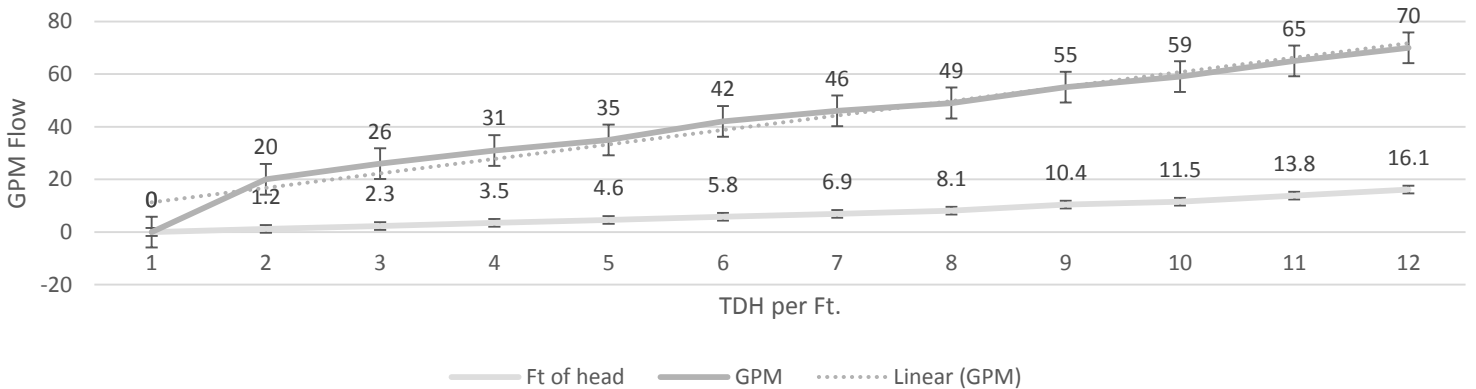
Head Loss
