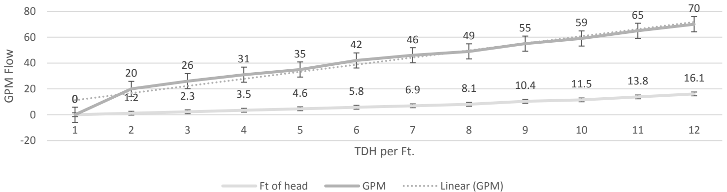
Head Loss
